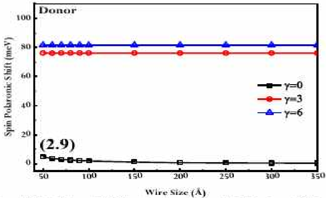
Figure 2.9: Spin Polaronic Shift due to the donor BMP vs Wire Size for x = 0.3 for various magnetic field.
