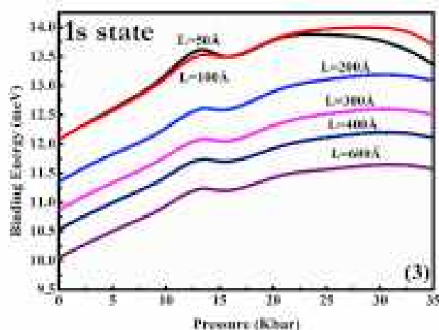
Fig. 3. Variation of binding energy of donor impurity against pressure for 1s state for various well widths.
