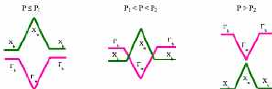
Fig. 2. Schematic band diagram for the \Gamma - X crossover due to the applied hydrostatic pressure in TQW.
