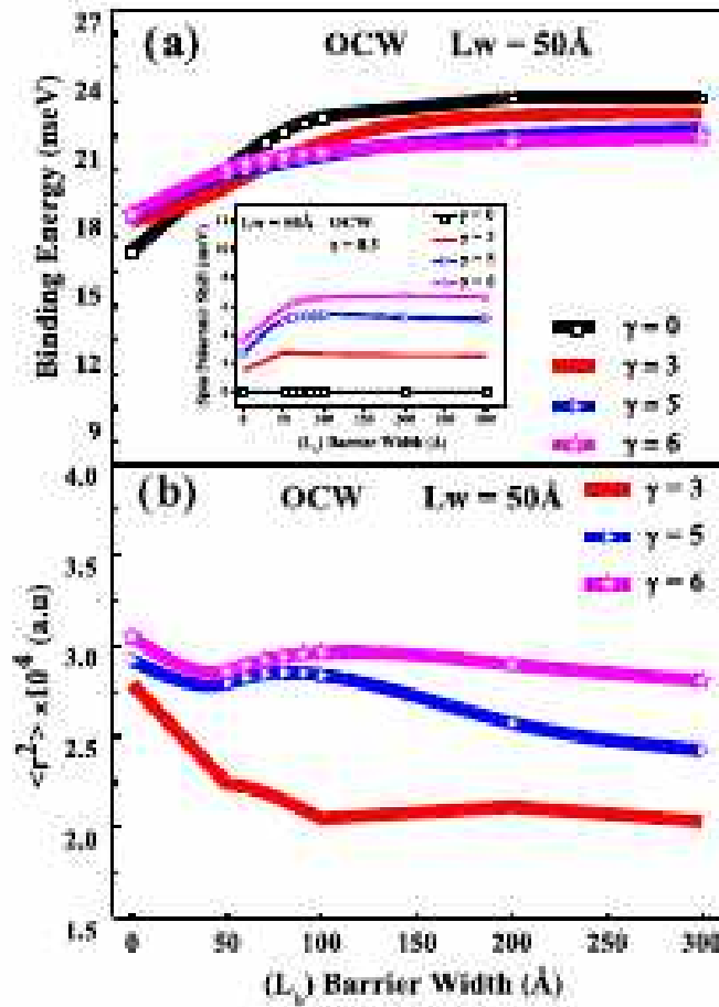
Fig. 3. Variation of (a) binding energy and (b) \langle r^2 \rangle against barrier width for lower well dimension L_w = 50 \text{ \AA} with the application of magnetic field ( \gamma = 0, 3 and 5 ) for the Mn ion concentration of x = 0.3 . Graphs have been plotted for OCW impurity.
