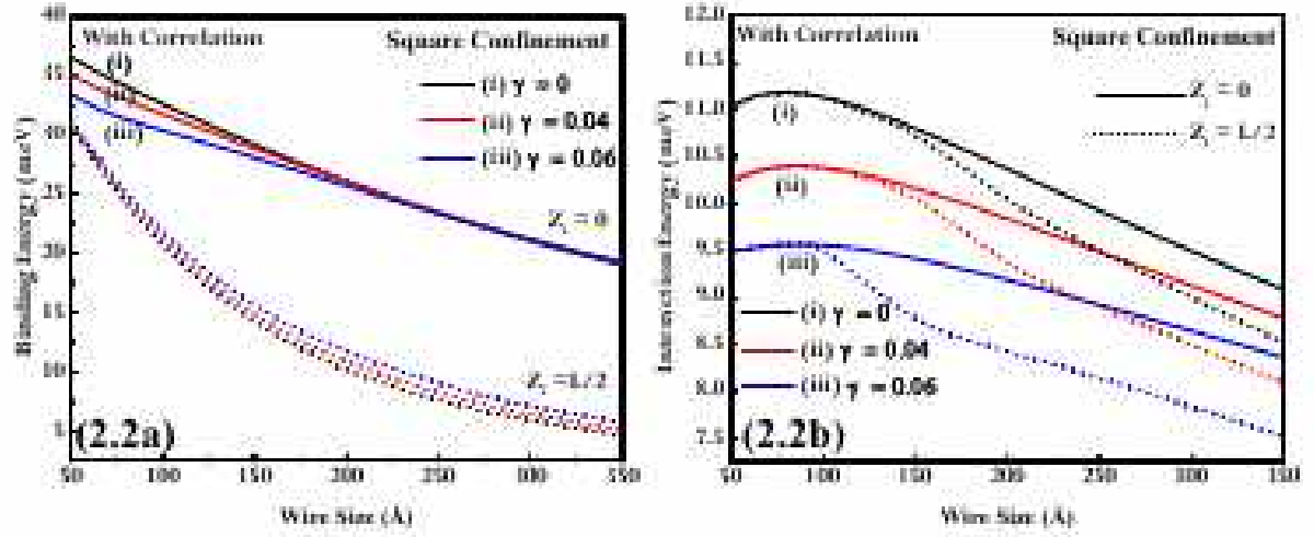
Figure 2.2: Variation of (a) binding energy and (b) interaction energy of the two holes bound to an acceptor impurity in a SQWW with square well type confining potential for different impurity locations and magnetic field by accounting the correlation between the carriers.
