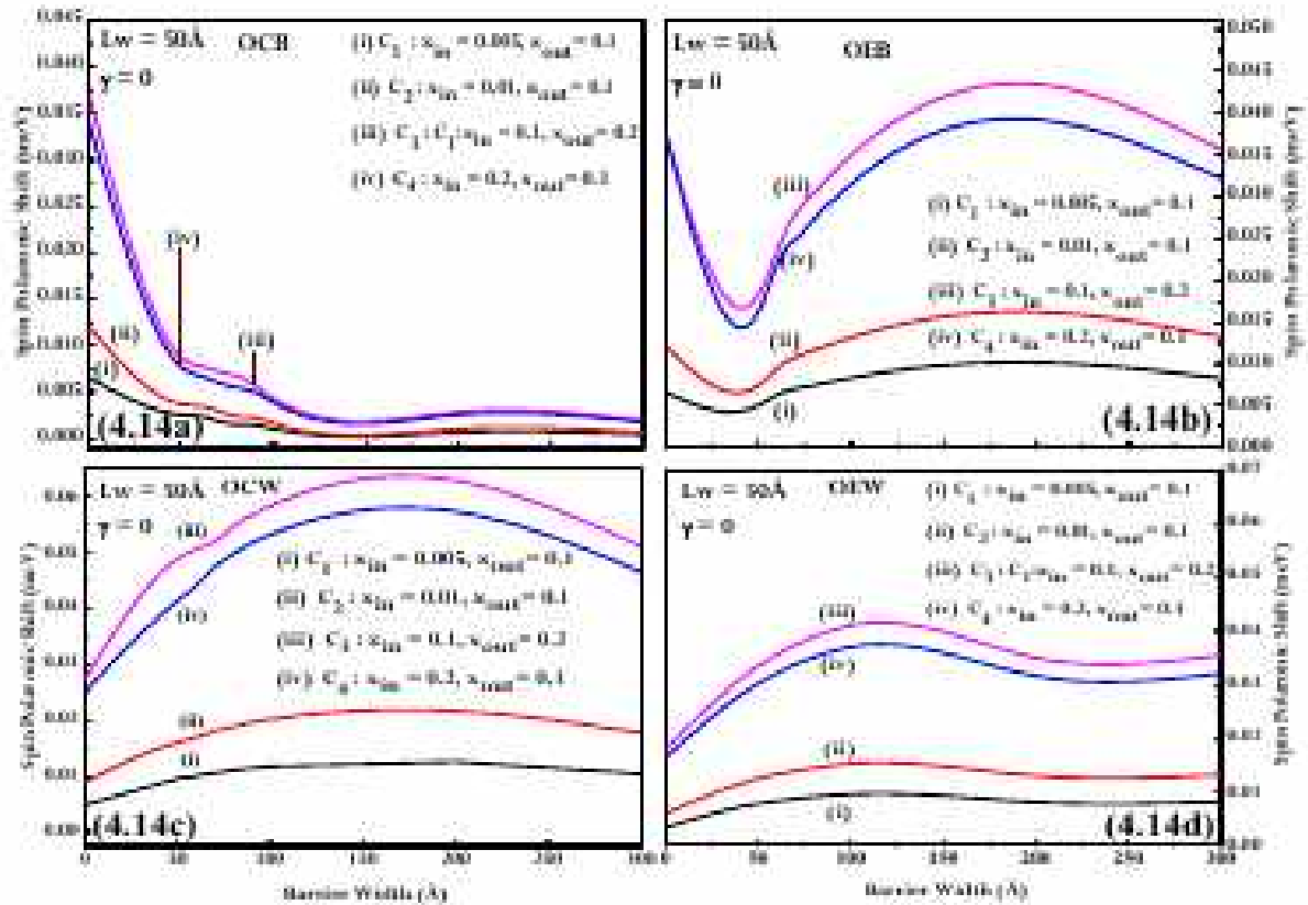
Figure 4.14: Variation of SPS against the barrier width for different combinations C_i of concentration of Mn^{2+} for composition of x = 0.1 ( x_{out} = x_{in} = C_i ) in a DQW with well width of L_w = 50 \text{ Å} for (a) OCB, (b) OEB, (c) OCW and (d) OEW impurities without the application of magnetic field ( \gamma = 0 ).
