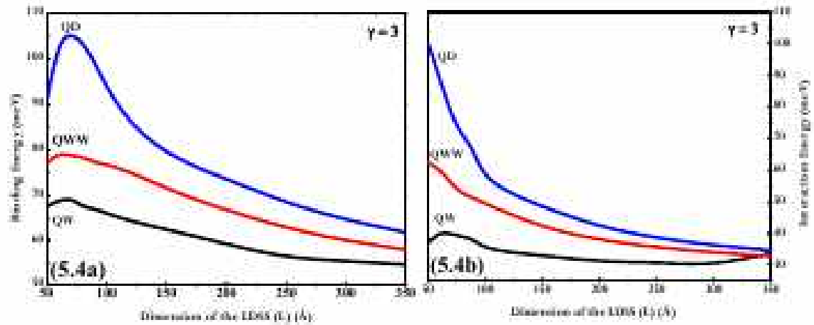
Figure 5.4: Variation of (a) binding energy and (b) interaction energy for the two electrons confined inside QW, QWW and QD as a function of dimension of the LDSS for the magnetic field \gamma = 3 .
