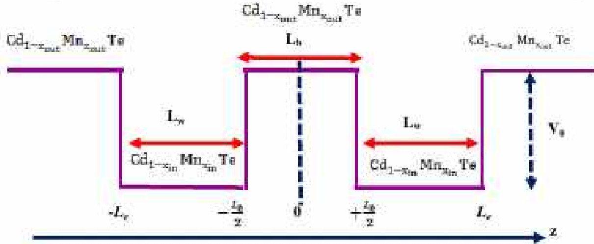
Figure 1: Schematic view of the potential profile for a DQW
