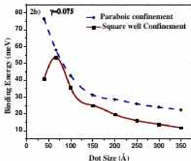
FIGURE 2b. Variation of binding energy of double acceptors vs. dot size for \gamma=0.075 .
