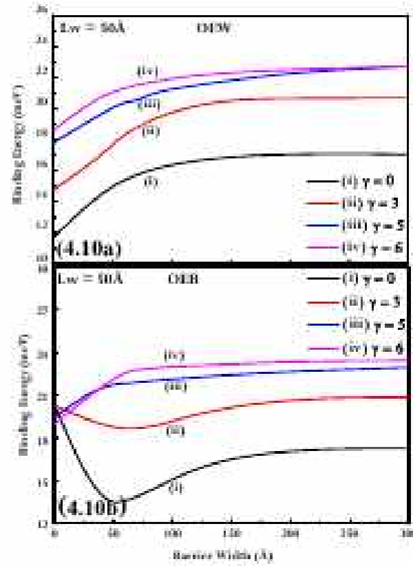
Figure 4.10: Variation of binding energy against barrier width for lower well dimension L_w = 50 \text{ \AA} with and without the application of magnetic field ( \gamma = 0, 3, 5 and 6 ) for the Mn ion concentration of x = 0.3 . Graphs have been plotted for (a) OEW and (b) OEB impurity.
