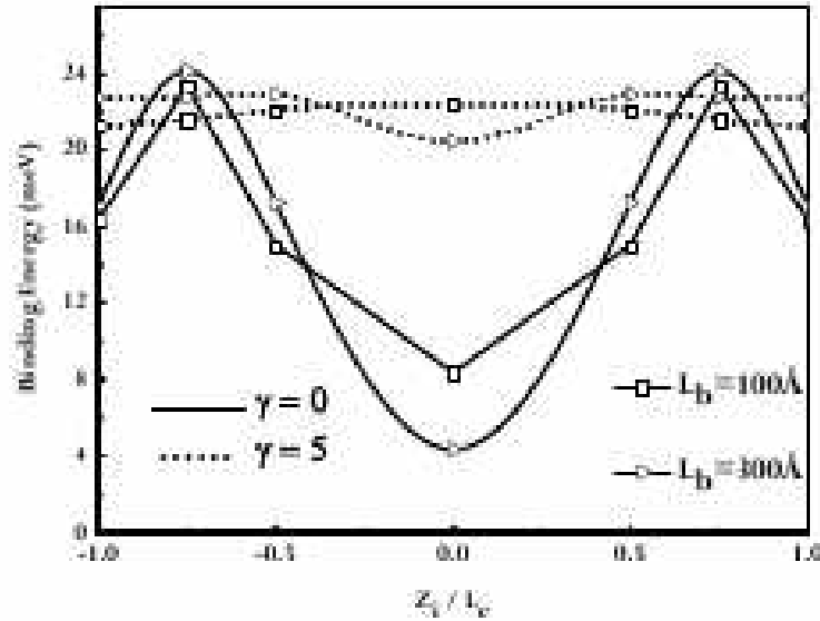
Figure 4.13: Variation of Binding energy as a function of impurity position is plotted for DQW with a well width of 50 \text{ Å} . The solid and dashed lines are corresponding to \gamma = 0 and \gamma = 5 respectively. The square and triangle symbols represents L_b = 100 \text{ Å} and L_b = 300 \text{ Å} respectively.
