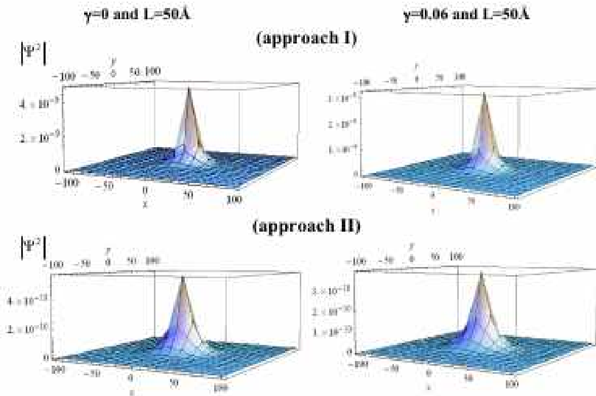
Figure 2.12: Probability distribution |\Psi^2| for heavy hole bound to an acceptor impurity inside the QWW of size L=50\text{\AA} under \gamma=0 and \gamma=0.06 for approach I and II.
