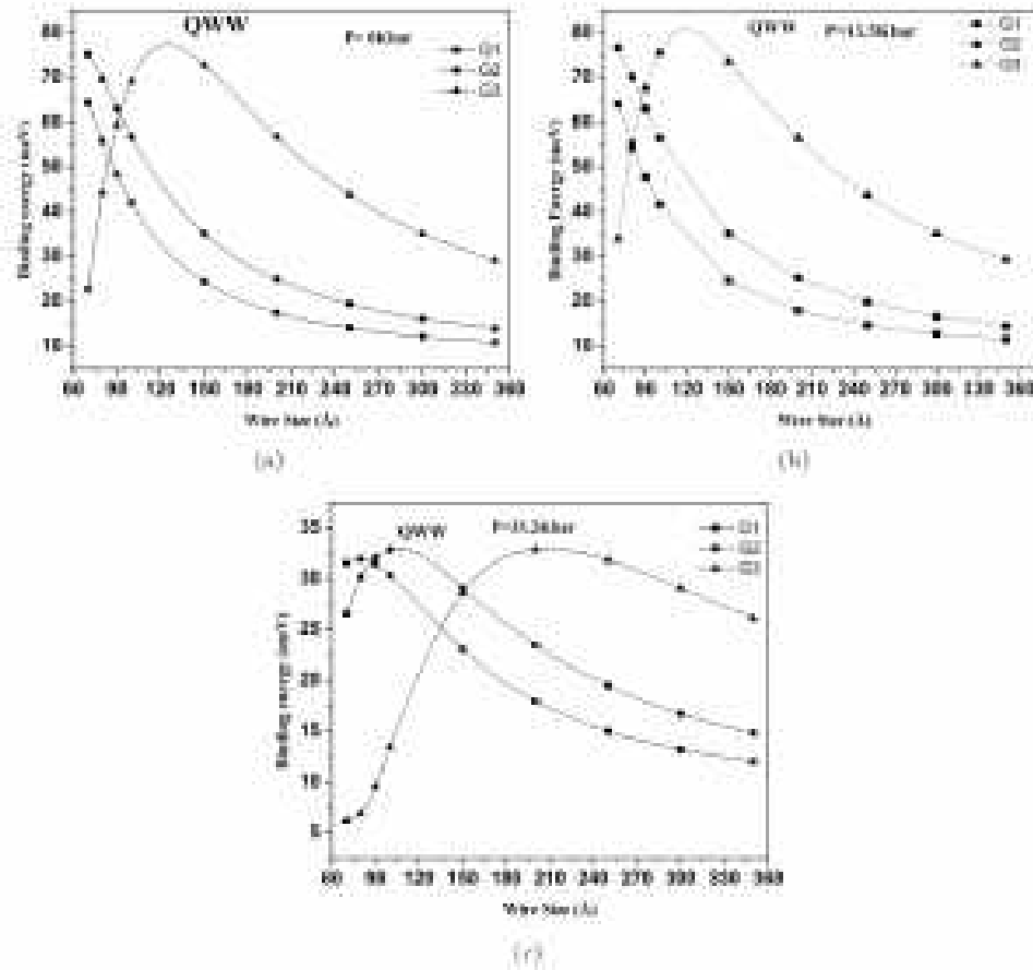
Fig. 3. Variation of donor binding energy as a function of wire size for three different pressure values of (a) P = 0 , (b) P = 13.5 and (c) 31.2 Kbar for various cross-sectional geometries.
