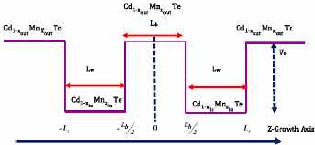
Figure 4.1: Schematic view of the potential profile for a DQW
