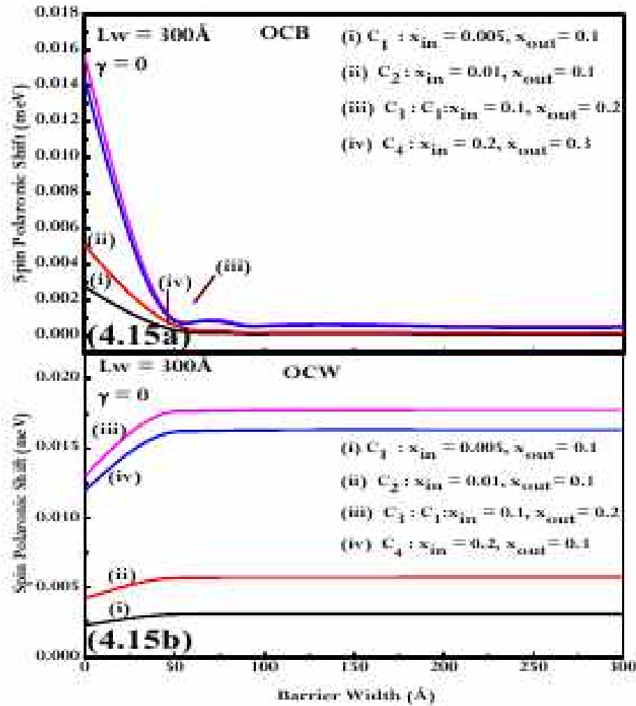
Figure 4.15: Variation of SPS against the barrier width for different combinations C_i of concentration of Mn^{2+} for composition of x = 0.1 ( x_{out} - x_{in} = C_i ) in a DQW with a well width of L_w = 300 \text{ Å} for (a) OCB, (b) OCW impurities without the application of magnetic field.
