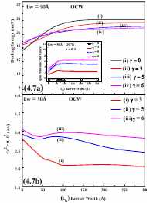
Figure 4.7: Variation of (a) binding energy and (b) \langle P^2 \rangle against barrier width for lower well dimension L_w = 50 Å with the application of magnetic field ( \gamma = 3, 5 and 6 ) for the Mn ion concentration of x = 0.3 . Graphs have been plotted for OCW impurity.
