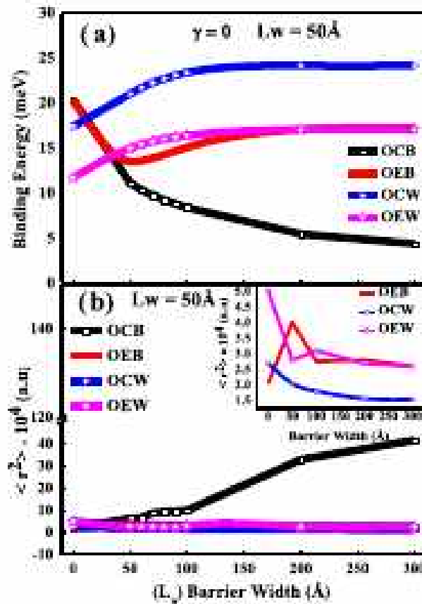
Fig. 2. Variation of (a) binding energy and (b) \langle r^2 \rangle against barrier width for lower well dimension L_w = 50 \text{ Å} without the application of magnetic field ( \gamma = 0 ) for the Mn ion concentration of x = 0.3 . Graphs have been plotted against various impurity locations ( x_i ).
