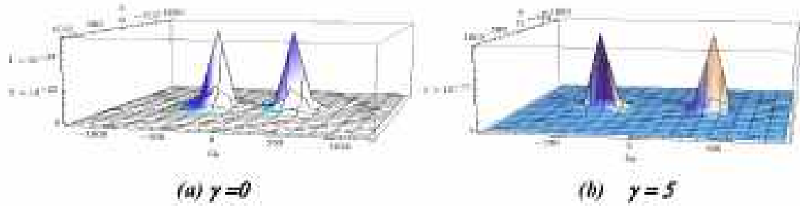
Figure 4.11: Probability density |\psi|^2 of the donor placed at OEW for various dimensions of the barrier and well under \gamma = 0 and \gamma = 5 for Mn ion concentration of x=0.3 .
