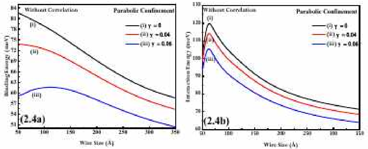
Figure 2.4: Carriers in Parabolic type confining potential. Variation of (a) binding energy and (b) interaction energy of the two holes bound to an acceptor impurity in a SQWW for various magnetic field by neglecting the correlation between the carriers.
