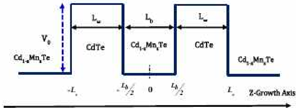
Figure 4.17: Schematic view of the potential profile of the valence band in DQW.
