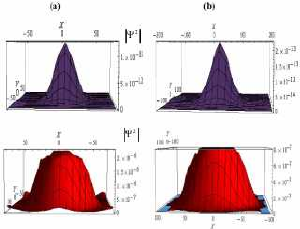
Figure 3.2: Probability distribution |\Psi^2| of the holes inside the QD of size 50\text{\AA} for (a) \gamma = 0 , (b) \gamma = 0.06 for cubical (Blue) and Spherical (Red) Quantum Dot.
