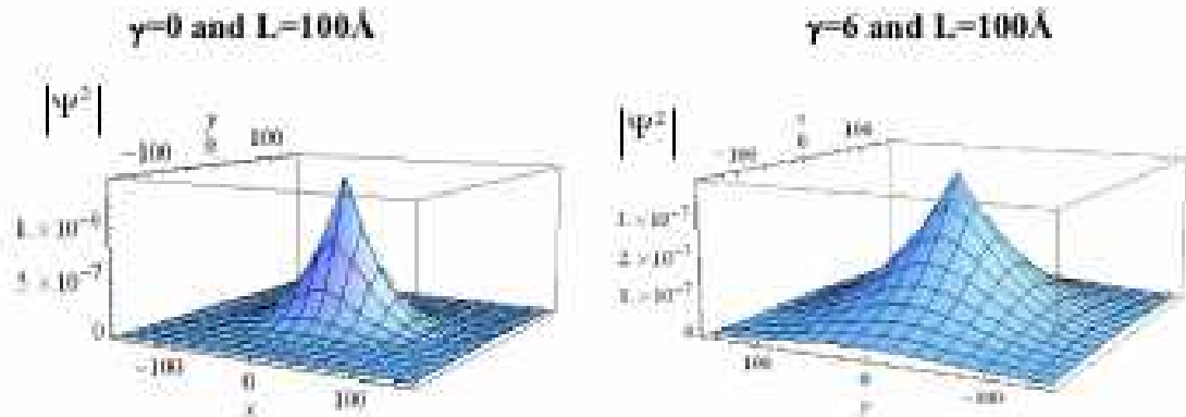
Figure 2.8: Probability distribution |\Psi^2| of the electron in a QWW under \gamma=0 and \gamma=6 for wire size L=100\text{\AA} .
