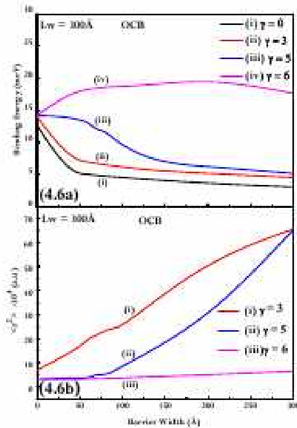
Figure 4.6: Variation of (a) binding energy and (b) \langle r^2 \rangle against barrier width for larger well dimension L_w = 300 \text{ Å} with the application of magnetic field ( \gamma = 3, 5 and 6 ) for the Mn ion concentration of x = 0.3 . Graphs have been plotted for OCB impurity.
