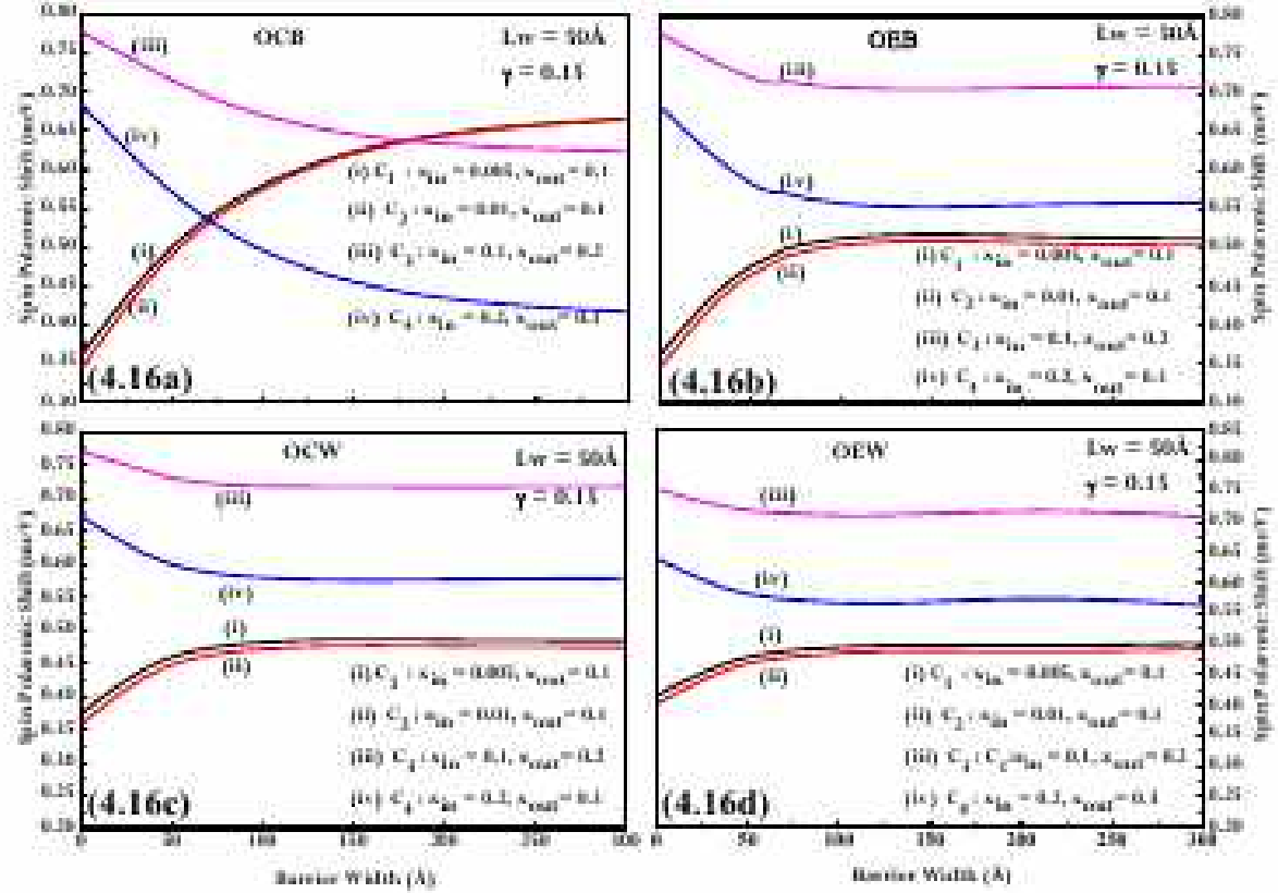
Figure 4.16: Variation of SPS against the barrier width for different combinations C_i of Mn^{2+} composition of x = 0.1 in a DQW with L_w = 50 \text{ Å} for (a) OCB, (b) OEB, (c) OCW and (d) OEW impurities with the application of magnetic field ( \gamma = 0.15 ).
