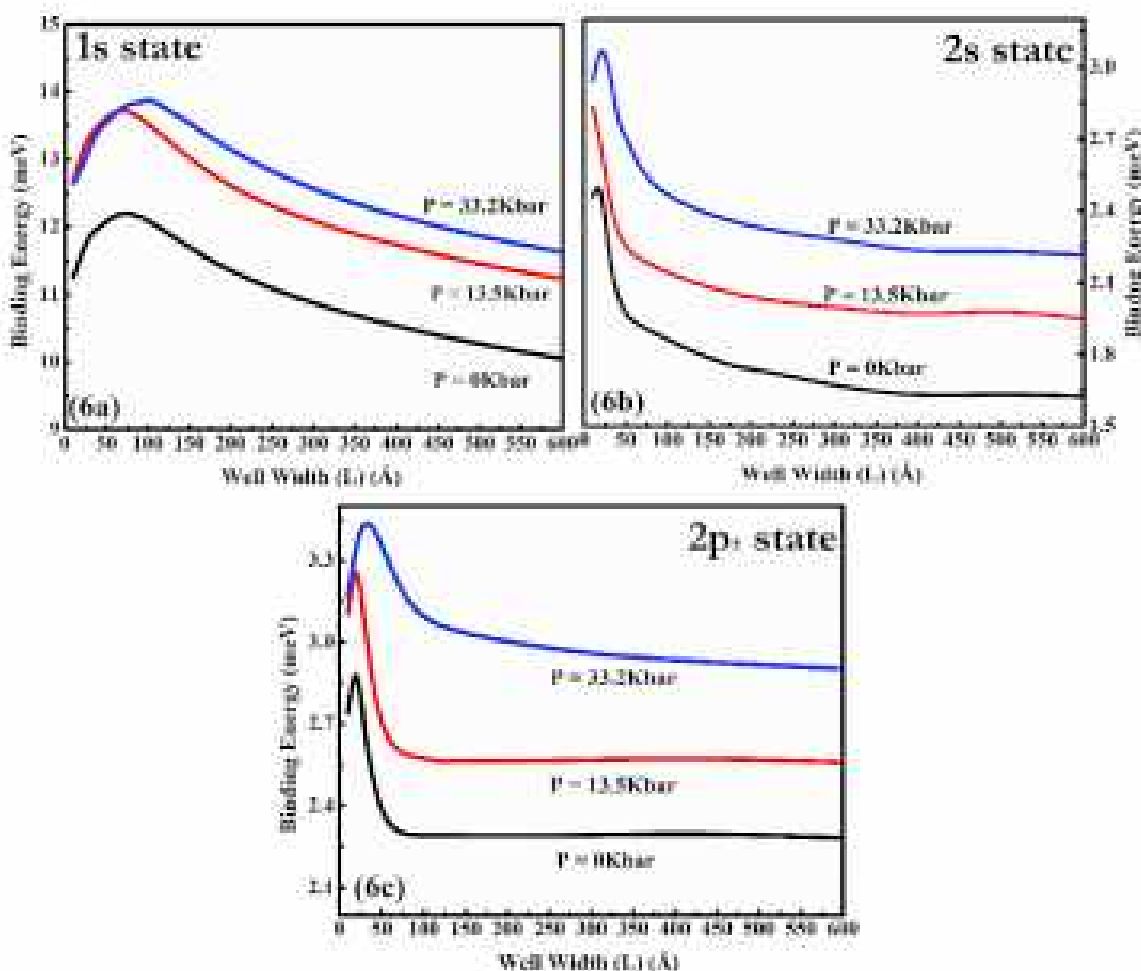
Fig. 6. Variation of binding energy of donor impurity against well width for (a) 1s state, (b) for 2s state and (c) for 2p z state for various pressures.
