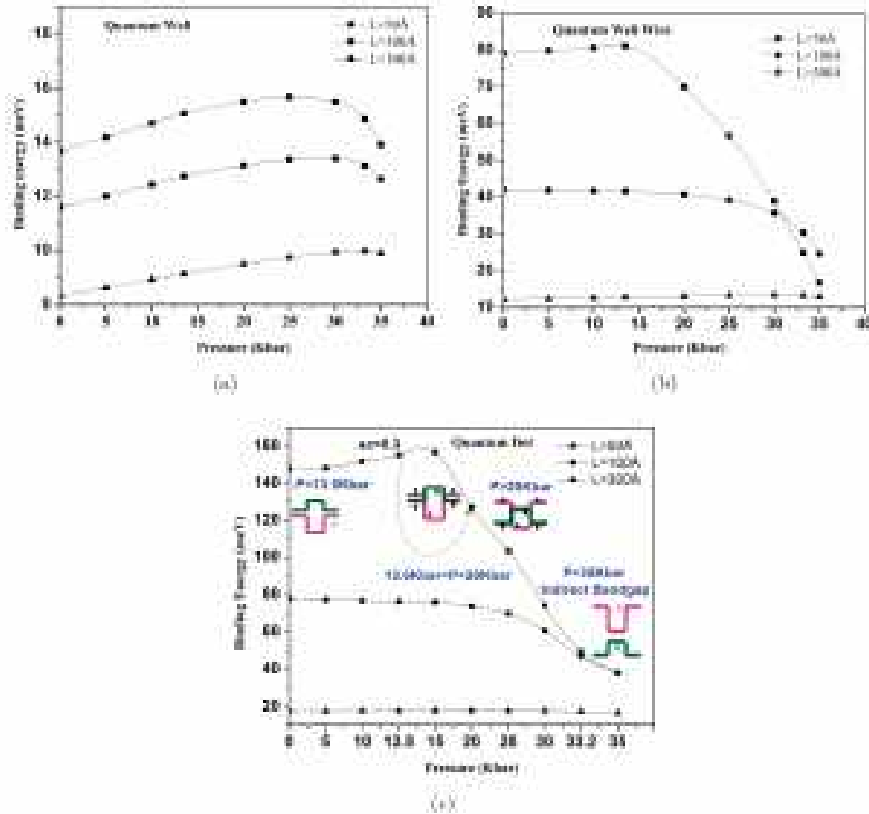
Fig. 1: Variation of donor binding energy as a function of pressure for (a) QW, (b) QWW and (c) QD.
