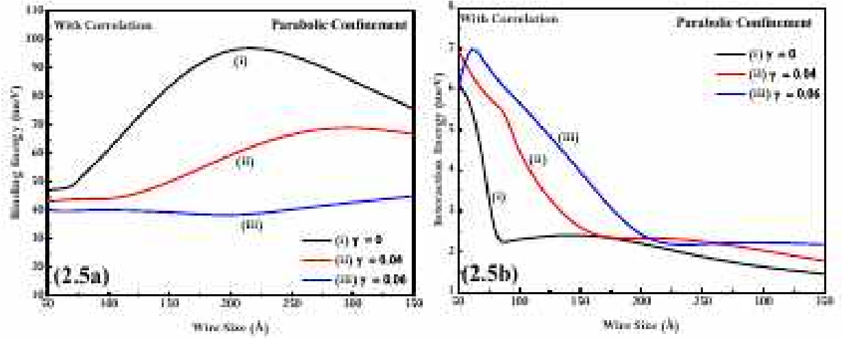
Figure 2.5: Carriers in Parabolic type confining potential. Variation of (a) binding energy and (b) interaction energy of the two holes bound to an acceptor impurity in a SQWW for various magnetic field by including the correlation between the carriers.
