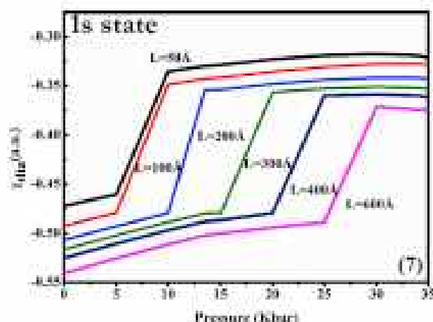
Fig. 7. Variation of \gamma_{1s} of donor impurity against pressure for 1s state for various well widths.
