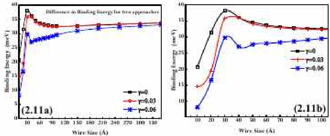
Figure 2.11: Difference in the acceptor binding energy between approach I and II as a function of wire size for various magnetic field. (a) Discrepancy shown for the whole range of the wire size and (b) shows for quite a large range of the narrow wires ( < 100\text{\AA} ).
