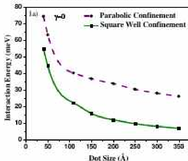
FIGURE 1a. Variation of Coulomb interaction of double acceptors vs. dot radius for \gamma=0 .
