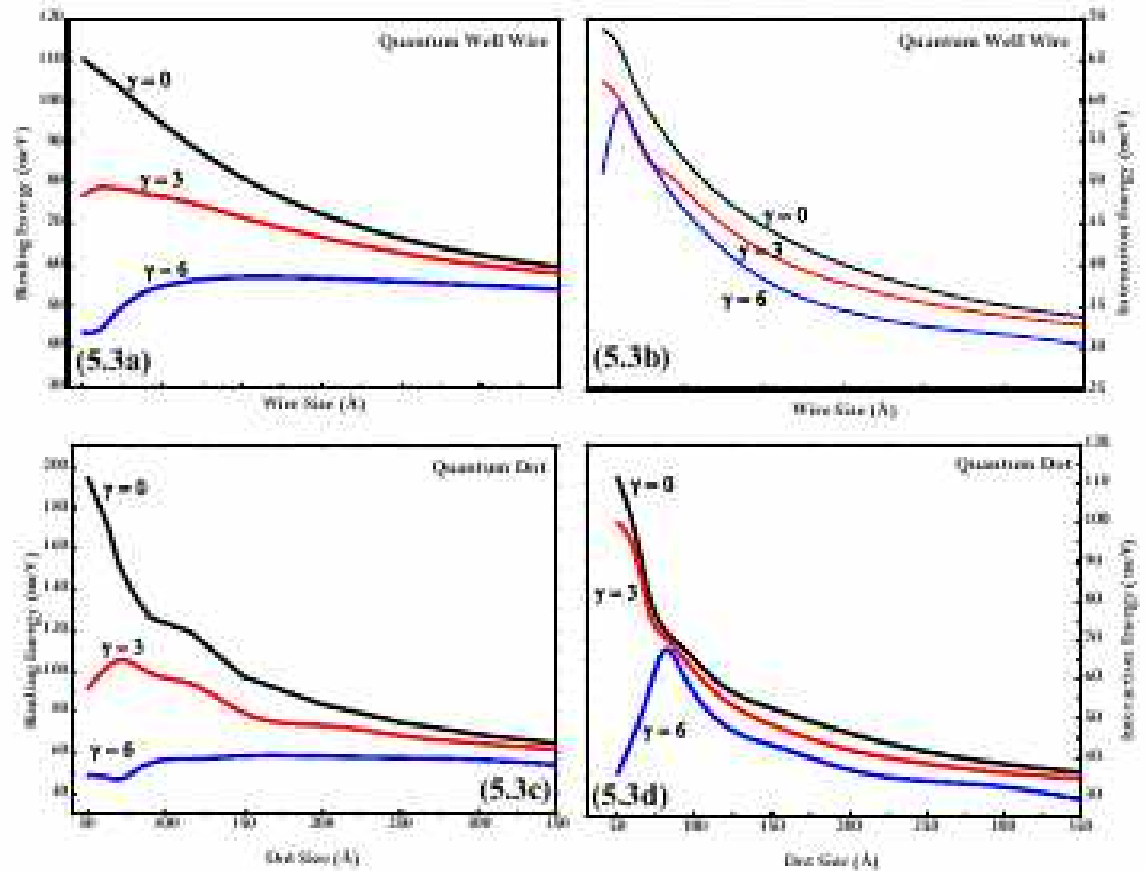
Figure 5.3: Variation of binding energy for the two electrons confined inside (a) QWW, (c) QD and the interaction energy in (b) QWW, (d) QD as a function of well width for different magnetic fields.
