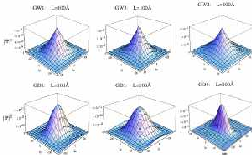
Fig. 6. 3D plot of |\Psi|^2 for various cross-sectional geometries of Quantum Well Wire and QD size L = 100 \text{ \AA} .
