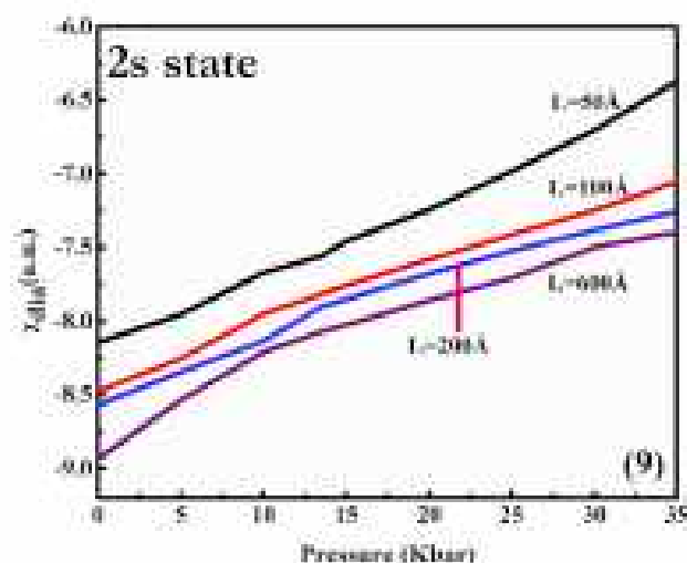
Fig. 9. Variation of \gamma_{2s} of donor impurity against pressure for 2s state for various well widths.
