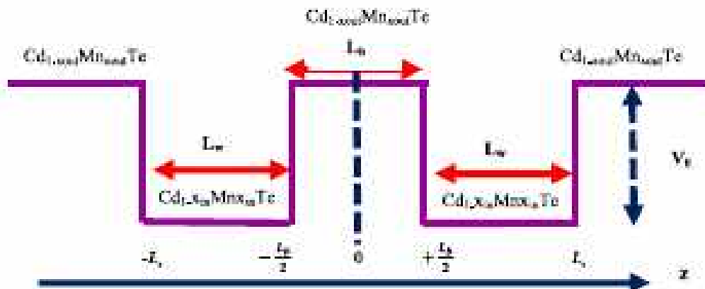
Fig. 1. Schematic view of the potential profile for a DQW.
