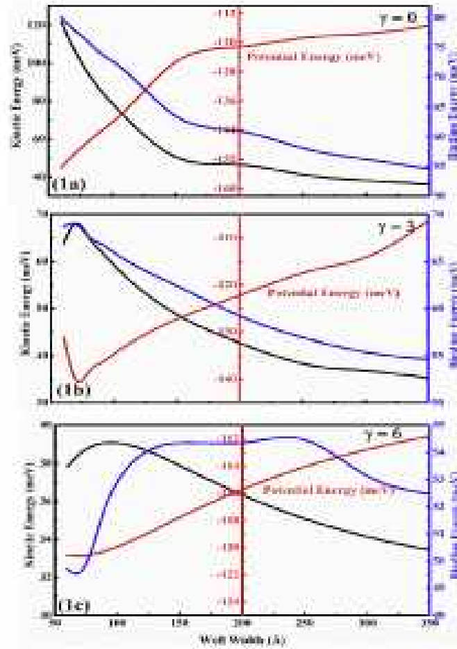
Fig. 1. Variation of Kinetic Energy, Potential energy and the Binding energy of the two electrons confined inside the QW as a function of well width for \gamma = 0 , \gamma = 3 and \gamma = 6 .
