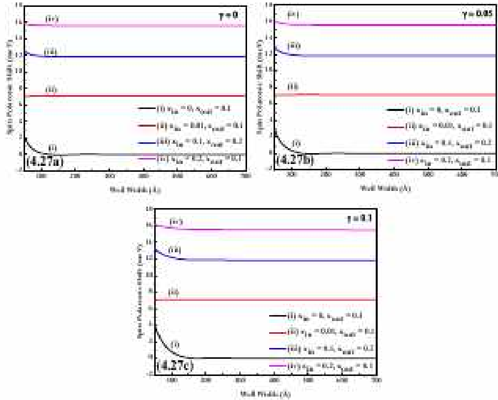
Figure 4.27: Variation of Spin Polaronic Shift against the well width for different combinations of concentration of Mn^{2+} for composition of x = 0.1 ( x_{out} - x_{in} = x = 0.1 ) in a STQW with and without the application of magnetic field (a) \gamma = 0 , (b) \gamma = 0.05 and (c) \gamma = 0.1 .
