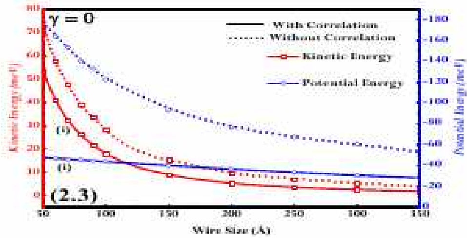
Figure 2.3: Comparison between the Case I and Case II by plotting kinetic energy and the potential energy variation against wire size for \gamma = 0 .
