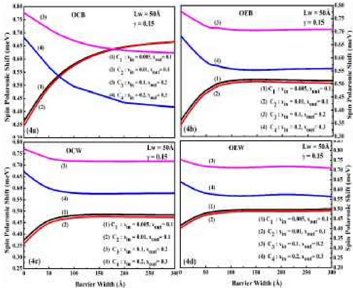
Figure 4: Variation of SPS against the barrier width for different combinations C_i of Mn^{2+} composition of x = 0.1 in a DQW with a well width of L_w = 50\text{\AA} for (a) OCB, (b) OEB, (c) OCW and (d) OEW impurities with the application of magnetic field ( \gamma = 0.15 ).
