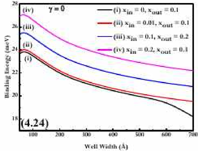
Figure 4.24: Variation of Binding Energy against the well width for different combinations of concentration of Mn^{2+} for composition of x = 0.1 ( x_{out} - x_{in} = x = 0.1 ) in a STQW without the application of magnetic field ( \gamma = 0 ).
