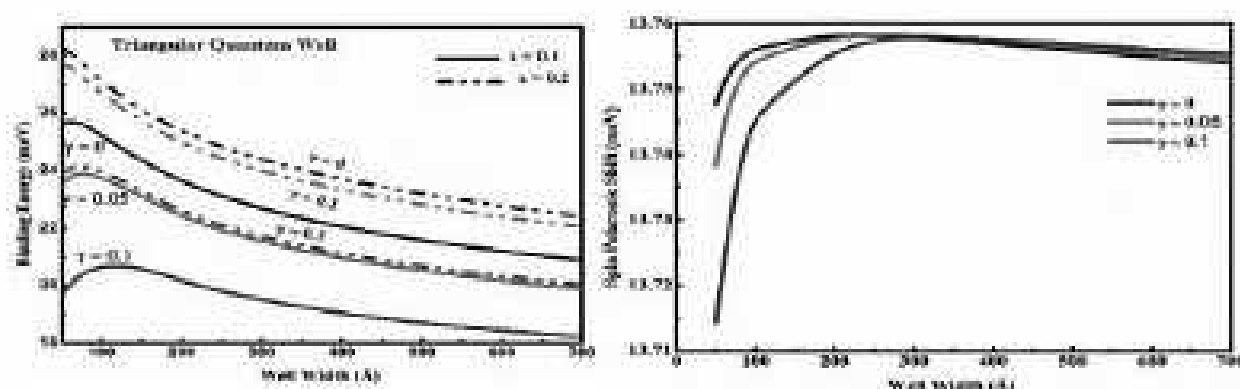
Fig 1. (a) Variation of Binding Energy for x = 0.1 and 0.2 , (b) SPS for x = 0.1 as a function of Well Width for various magnetic fields ( \gamma ).
