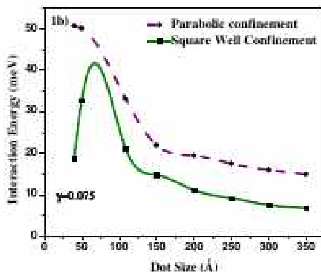
FIGURE 1b. Variation of Coulomb interaction of double acceptors vs. dot radius for \gamma=0.075 .
