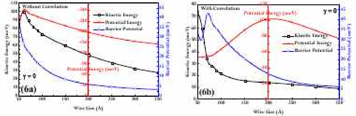
Figure 2.6: Comparison between the Case I and Case II by plotting kinetic energy and the potential energy variation against wire size for \gamma = 0 when carriers are confined in a parabolic potential. (a) Without including the Correlation and (b) With including the correlation.
