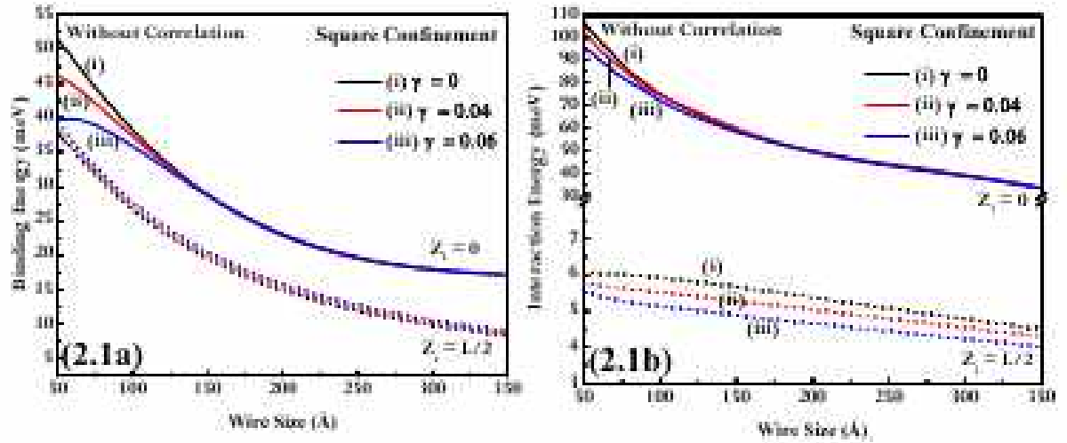
Figure 2.1: Variation of (a) binding energy and (b) interaction energy of the two holes bound to an acceptor impurity in a SQWW with square well type confining potential for different impurity locations and magnetic field by neglecting the correlation between the carriers.
