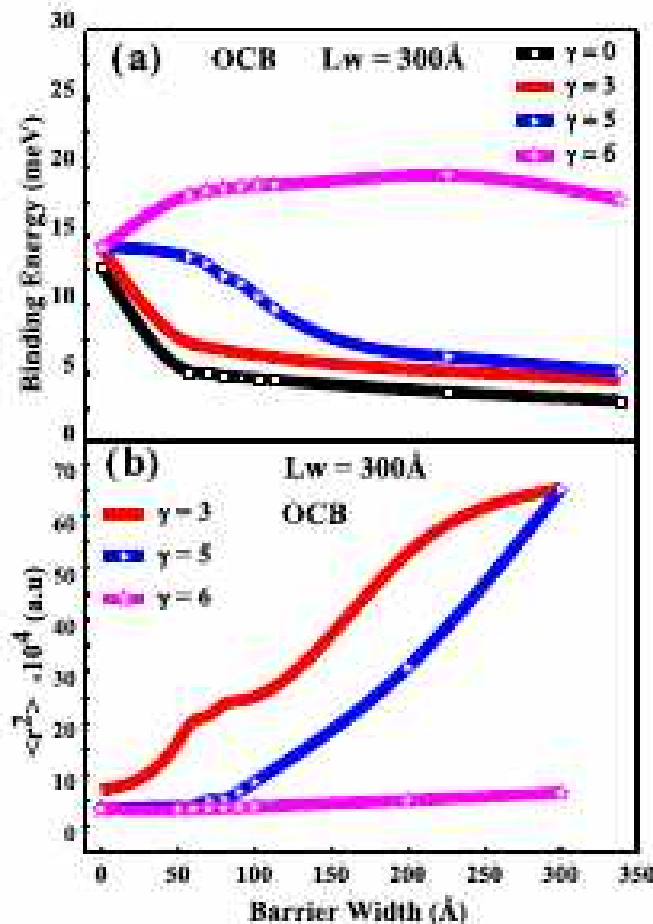
Fig. 6. Variation of (a) binding energy and (b) \langle r^2 \rangle against barrier width for larger well dimensions L_w = 300 \text{ \AA} with the application of magnetic field ( \gamma = 3, 5 and 6 ) for the Mn ion concentration of x = 0.3 . Graphs have been plotted for OCB impurity.
