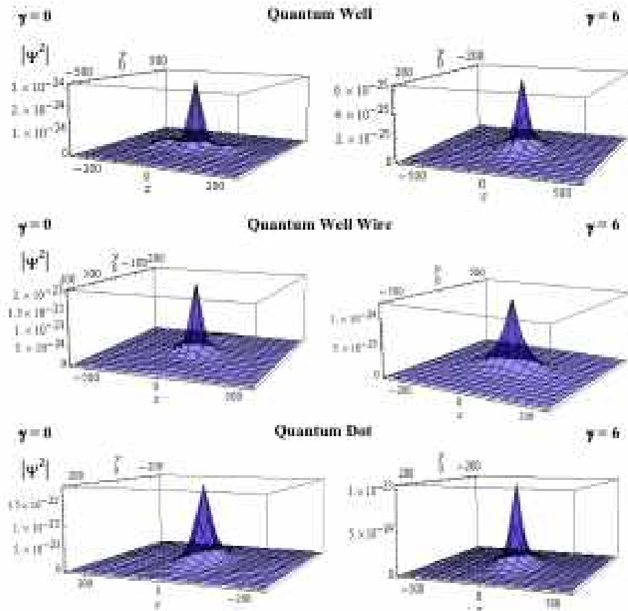
Fig. 5. Probability density |\Psi^2| of the 1s – 18s impurity confined inside the QW, QWW and QD under \gamma = 0 and \gamma = 6 for Na atom concentration of x = 0.1 .
