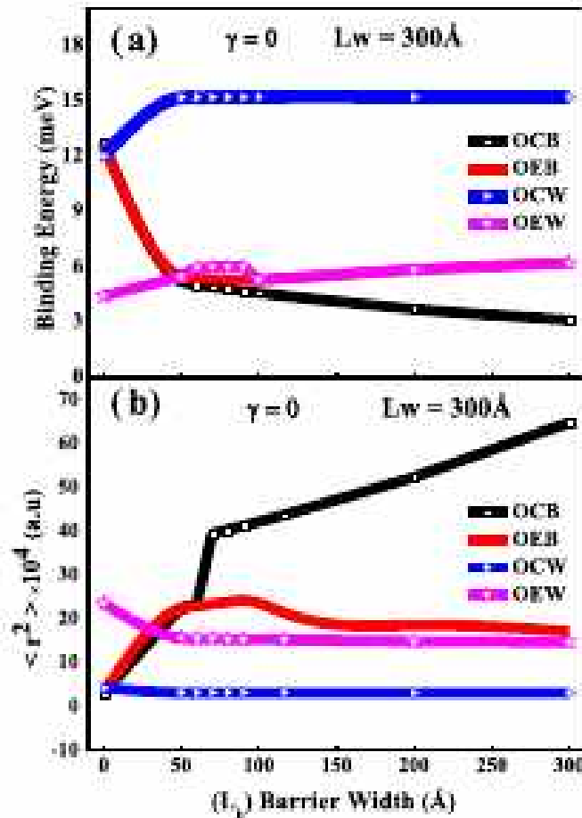
Fig. 3. Variation of (a) binding energy and (b) \langle r^2 \rangle against barrier width for larger well dimensions L_w = 300 Å without the application of magnetic field ( \gamma = 0 ) for the Mn ion concentration of x = 0.3 . Graphs have been plotted against various impurity locations ( \alpha_i ).
