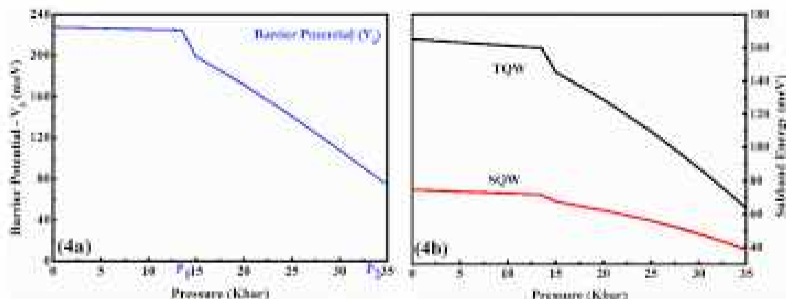
Fig. 4. (a) Variation of Confining Potential of TQW and (b) comparison of Subband Energy of TQW and SQW against Pressure.
