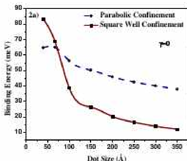
FIGURE 2a. Variation of binding energy of double acceptors vs. dot size for \gamma=0 .
