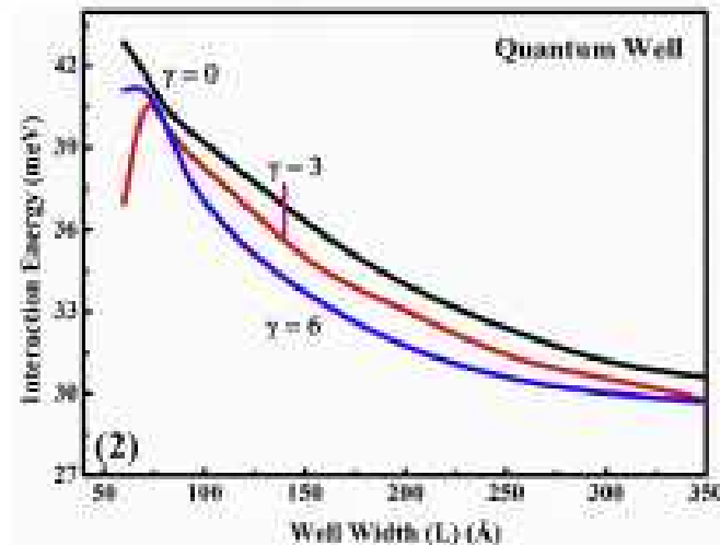
Fig. 2. Variation of interaction energy of the two electrons confined inside the QW as a function of well width for (a) \gamma = 0 , \gamma = 3 and (c) \gamma = 6 .
