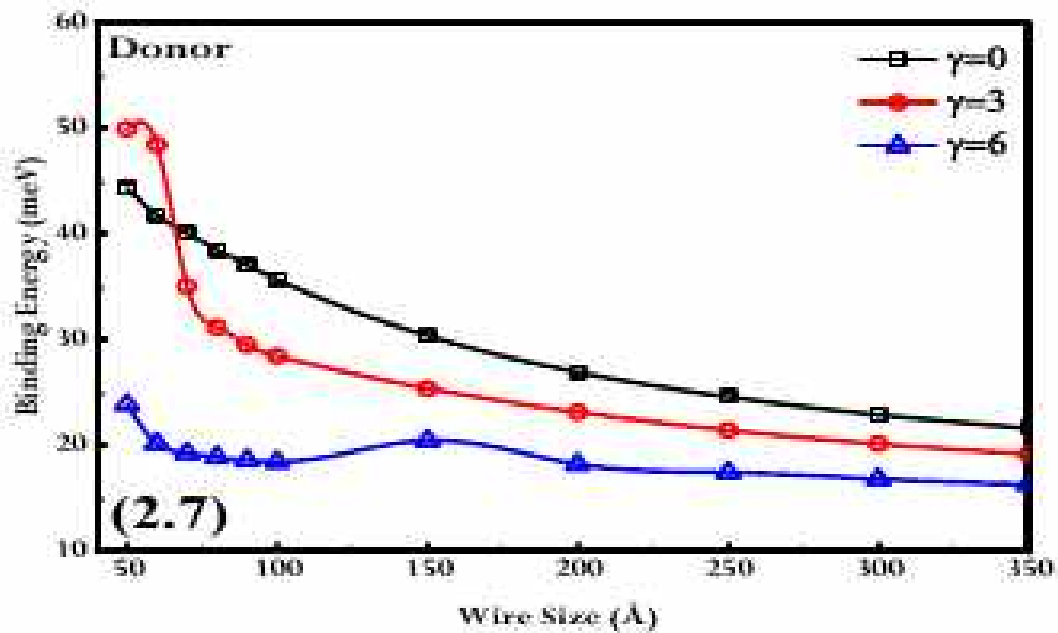
Figure 2.7: Donor Binding Energy vs Wire Size for x=0.3 for various magnetic field.
