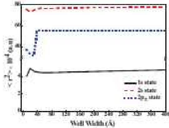
FIGURE 3. Variation of \langle r^2 \rangle of the donor impurity against well width.
