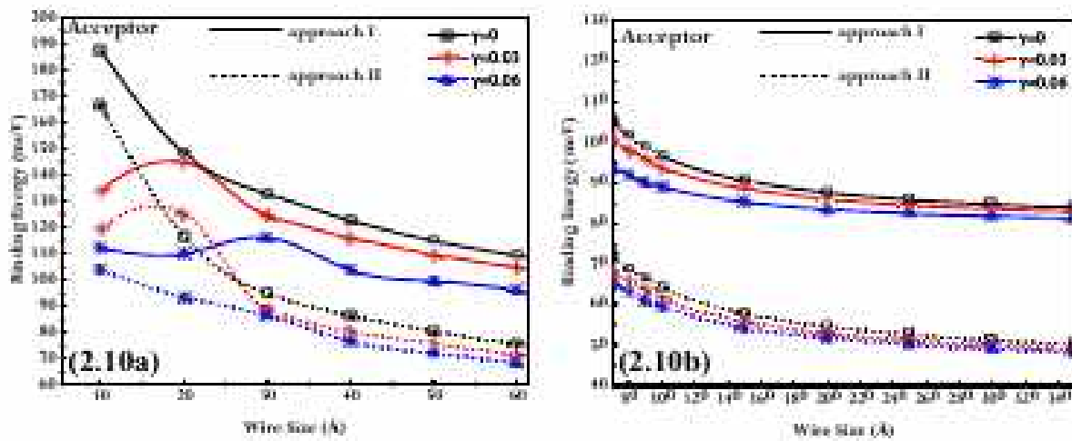
Figure 2.10: Variation of acceptor binding energy as a function of wire size for various magnetic field in approach I and II. Variation shows (a) for quite a large range of the narrow wires i.e. less than 60 Å and (b) for the wire size limited towards the bulk limit.
