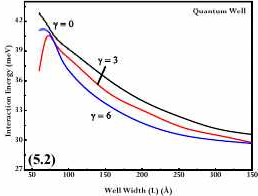
Figure 5.2: Variation of interaction energy of the two electrons confined inside the QW as a function of well width for \gamma = 0 , \gamma = 3 and \gamma = 6 .
