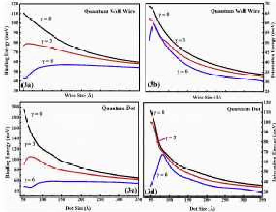
Fig. 3. Variation of binding energy for the two electron confined nano (a) QWW, (c) QD and the interaction energy in (b) QWW, (d) QD as a function of well width for different magnetic fields.
