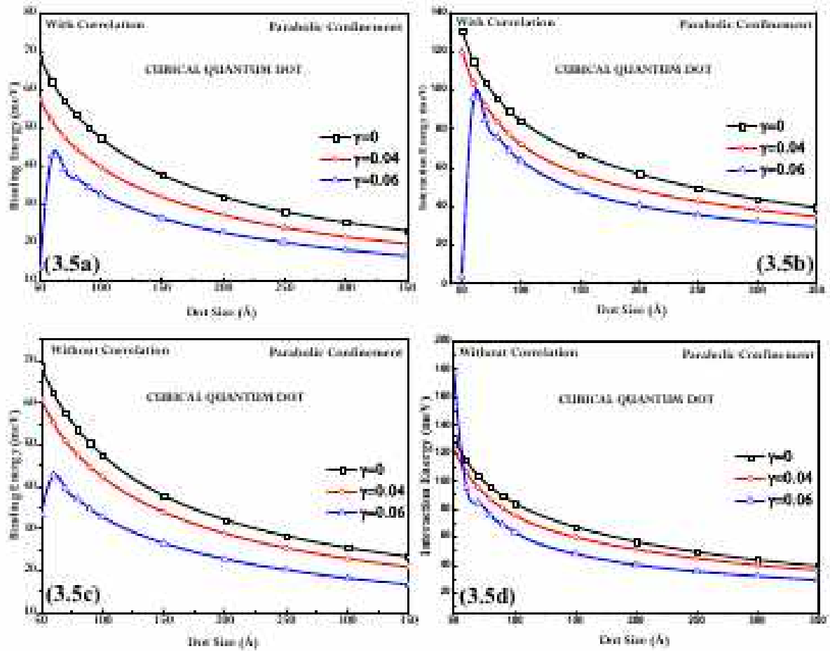
Figure 3.5: Variation of binding energy and E_{BH} as a function of dot size for CQD with parabolic confining potential under various applied magnetic field for both the inclusion and exclusion of the correlation between the two holes.
