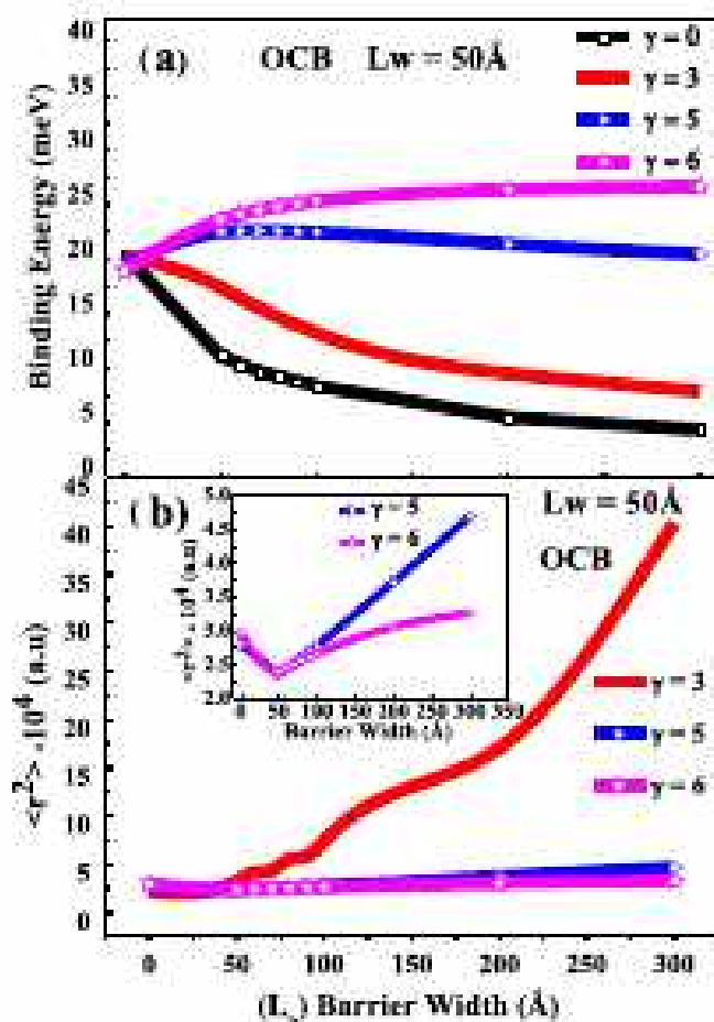
Fig. 4. Variation of (a) binding energy and (b) \langle r^{-2} \rangle against barrier width for lower well dimension L_w = 50 \text{ \AA} with the application of magnetic field \gamma = 0, 3 and 6 for the Mn ion concentration of x = 0.3 . Graphs have been plotted for OCB inequality.
