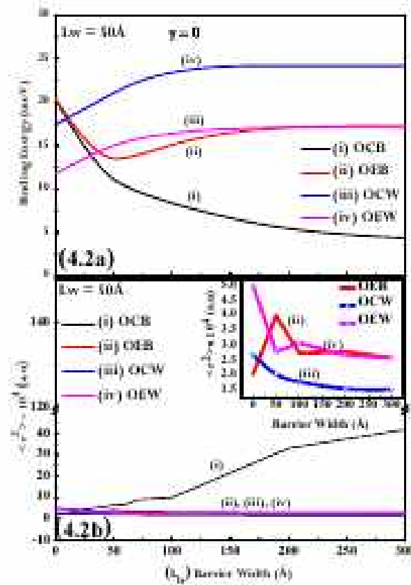
Figure 4.2: Variation of (a) binding energy and (b) \langle r^2 \rangle against barrier width for lower well dimension L_w = 50 Å without the application of magnetic field ( \gamma = 0 ) for the Mn concentration of x = 0.3 . Graphs have been plotted against various impurity locations ( z_i ).
