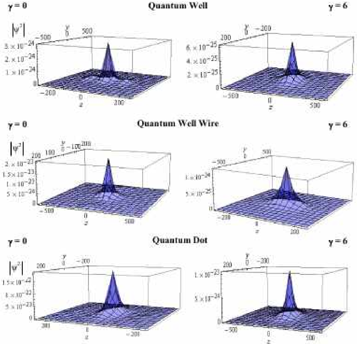
Figure 5.5: Probability density |\Psi^2| of the He-like impurity confined inside the QW, QWW and QD under \gamma = 0 and \gamma = 6 for Mn ion concentration of x=0.3 .
