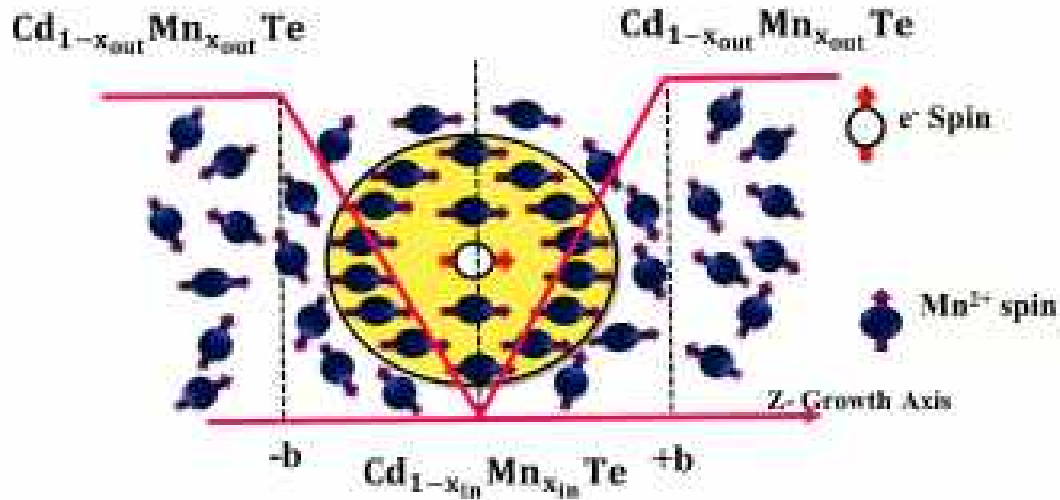
Figure 4.23: Formation of Bound Magnetic Polaron (BMP) in a Semimagnetic Triangular Quantum Well (STQW).
