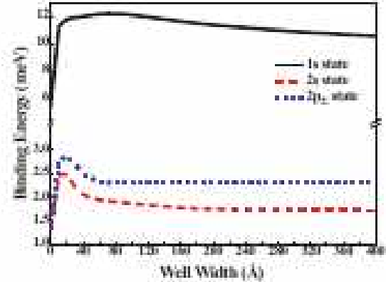
FIGURE 1. Variation of binding energy of donor impurity against well width for ground and low lying excited states.
