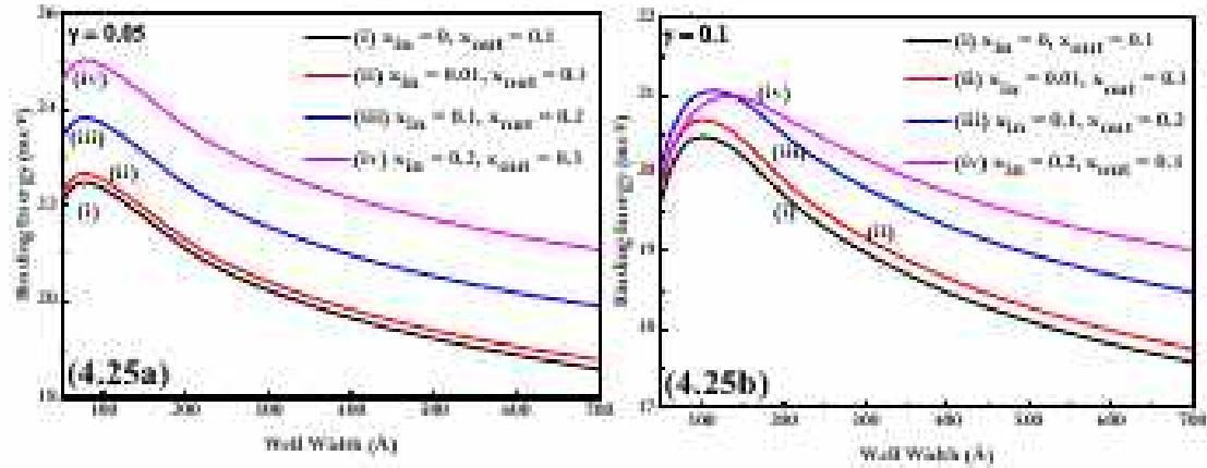
Figure 4.25: Variation of Binding Energy against the well width for different combinations of concentration of \text{Mn}^{2+} for composition of x = 0.1 ( x_{\text{out}} - x_{\text{in}} = x = 0.1 ) in a STQW with the application of magnetic field (a) \gamma = 0.05 and (b) \gamma = 0.1 .
